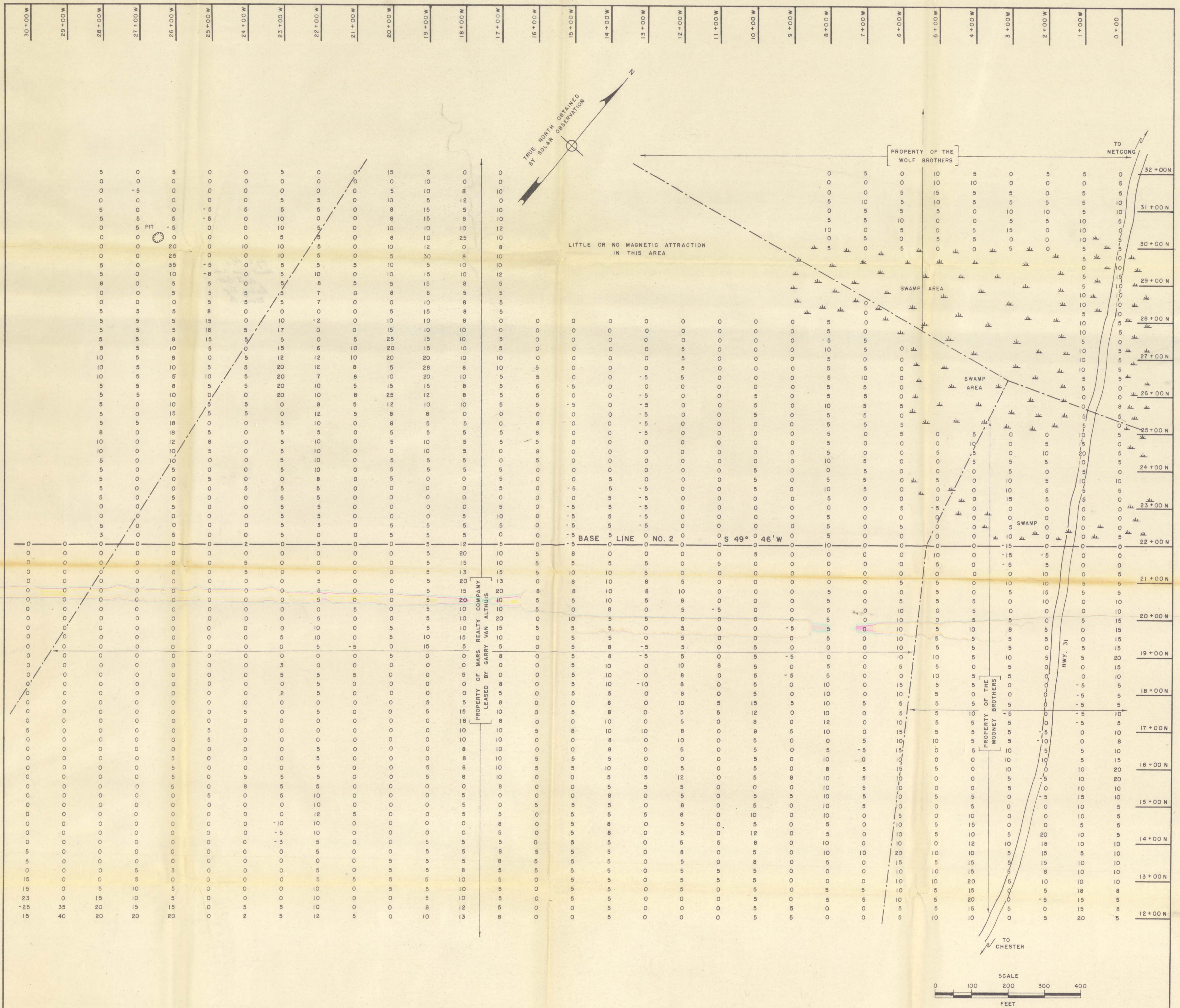
FIGURE 2 — PLATE 5 — DIP NEEDLE SURVEY MT. OLIVE AREA — NORTH BELT ROXBURY TOWNSHIP, MORRIS COUNTY, NEW JERSEY
