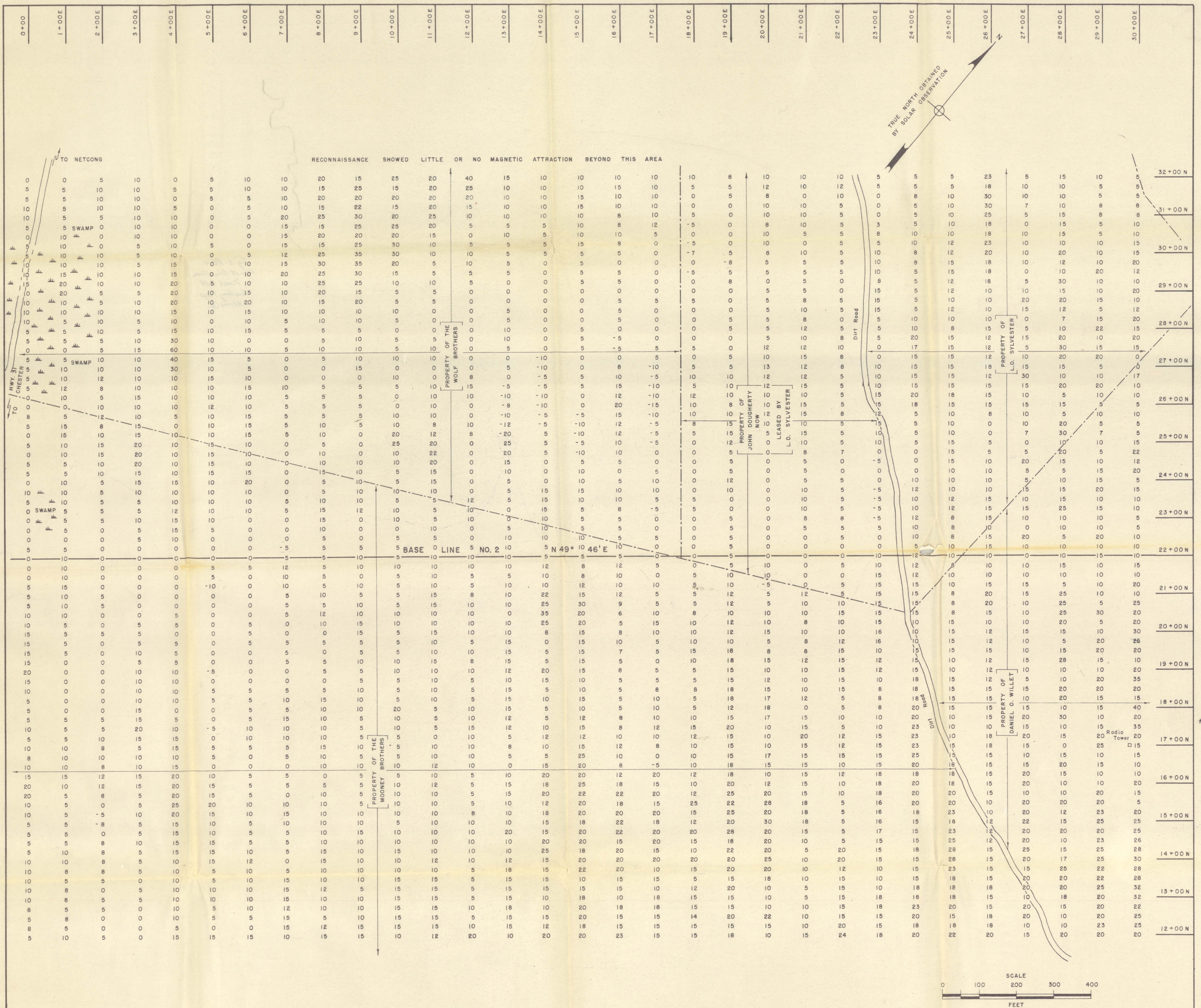
FIGURE 2 — PLATE 4 — DIP NEEDLE SURVEY MT. OLIVE AREA — NORTH BELT ROXBURY TOWNSHIP, MORRIS COUNTY, NEW JERSEY
