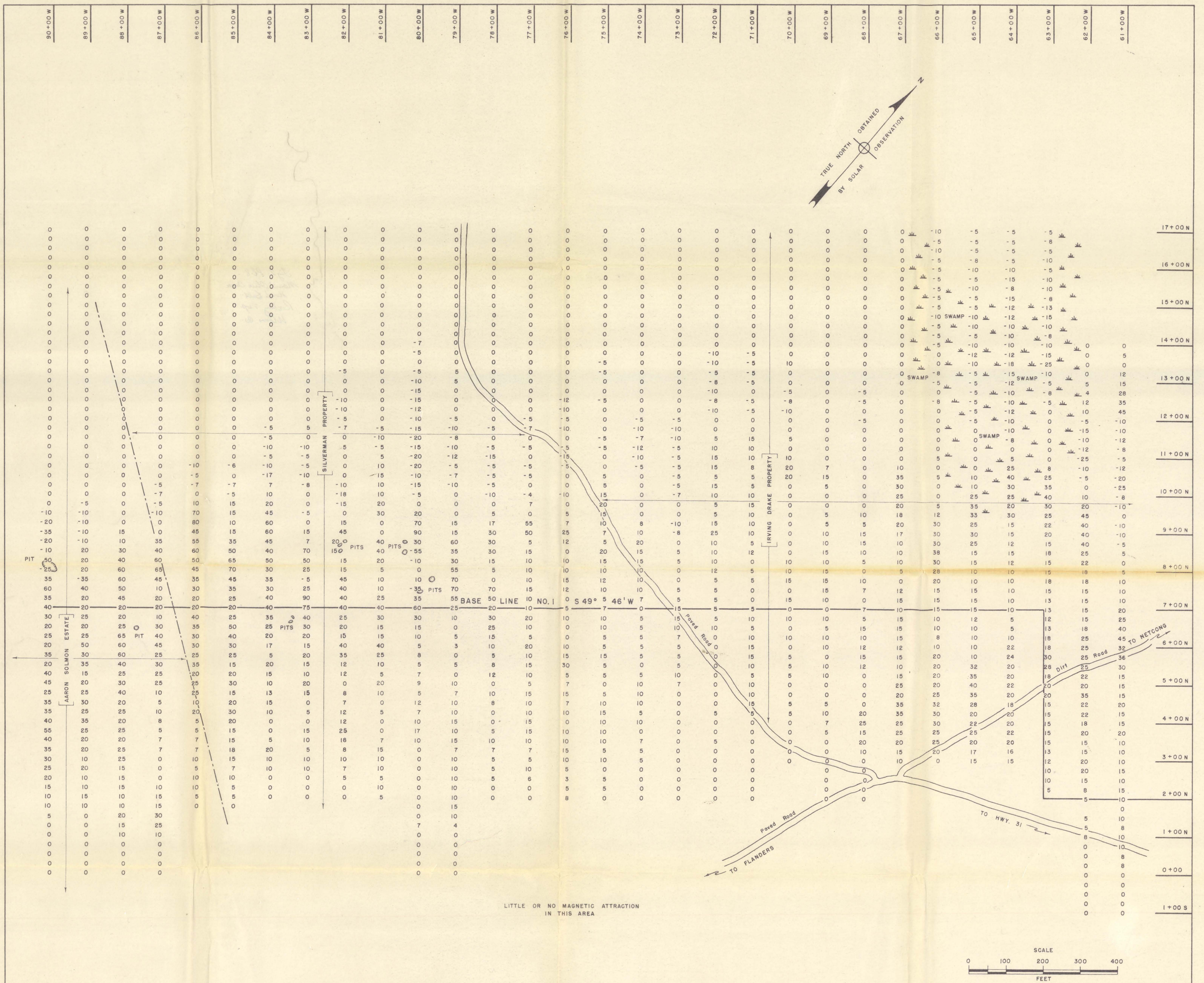
FIGURE 2 — PLATE 8 — DIP NEEDLE SURVEY MT. OLIVE AREA — NORTH BELT ROXBURY TOWNSHIP, MORRIS COUNTY, NEW JERSEY
