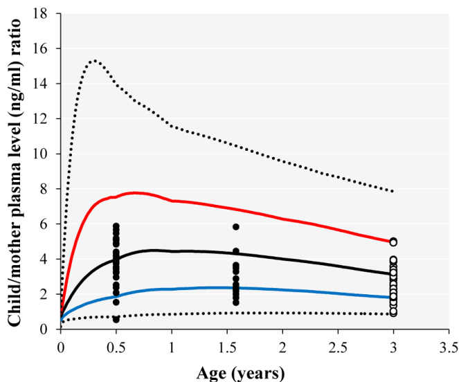
From Verner et al. (2016). Modeling simulation of the ratio of PFOA in blood plasma in breast fed infants/children to plasma concentration in mother. Black line - 50th percentile. Blue line - 5th percentile. Red line - 95th percentile. Dotted lines - minimum and maximum values.
