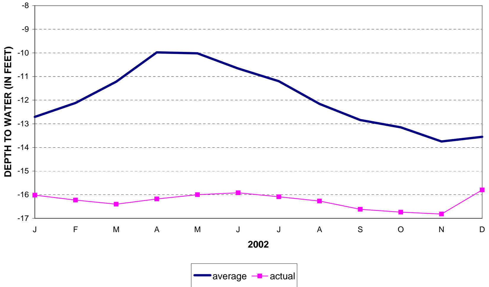
FIGURE 9: USGS WELL-NEW CASTLE CO., DELAWARE Average Vs. Actual 2002
