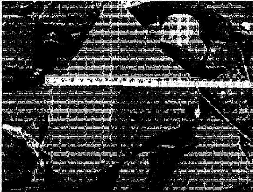
Figure 2: Measurement and type of existing riprap stone.
