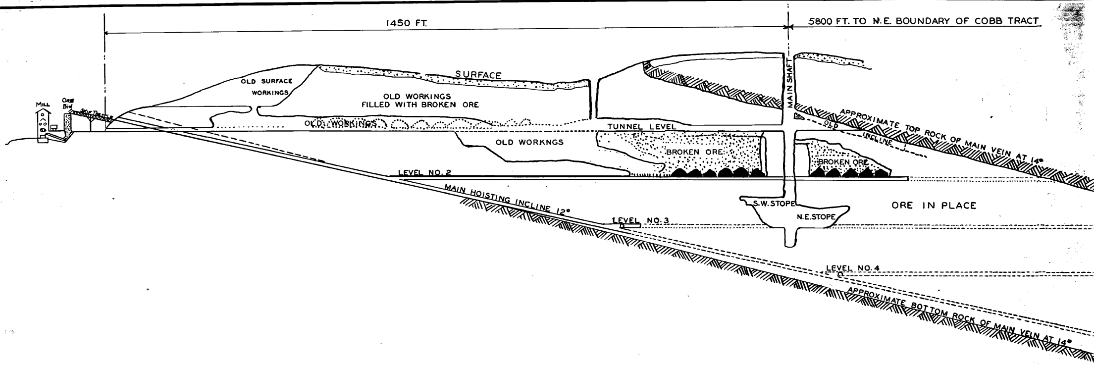
FIGURE U.S. DEPARTMENT OF THE INTERIOR BUREAU OF MINES SECOND EASTERN DISTRICT LONGITUDINAL SECTION SHOWING OLD WORKINGS AND PROPOSED DEVELOPMENT OF BEACH GLEN MINE SCALE 1" = 100 FT.
