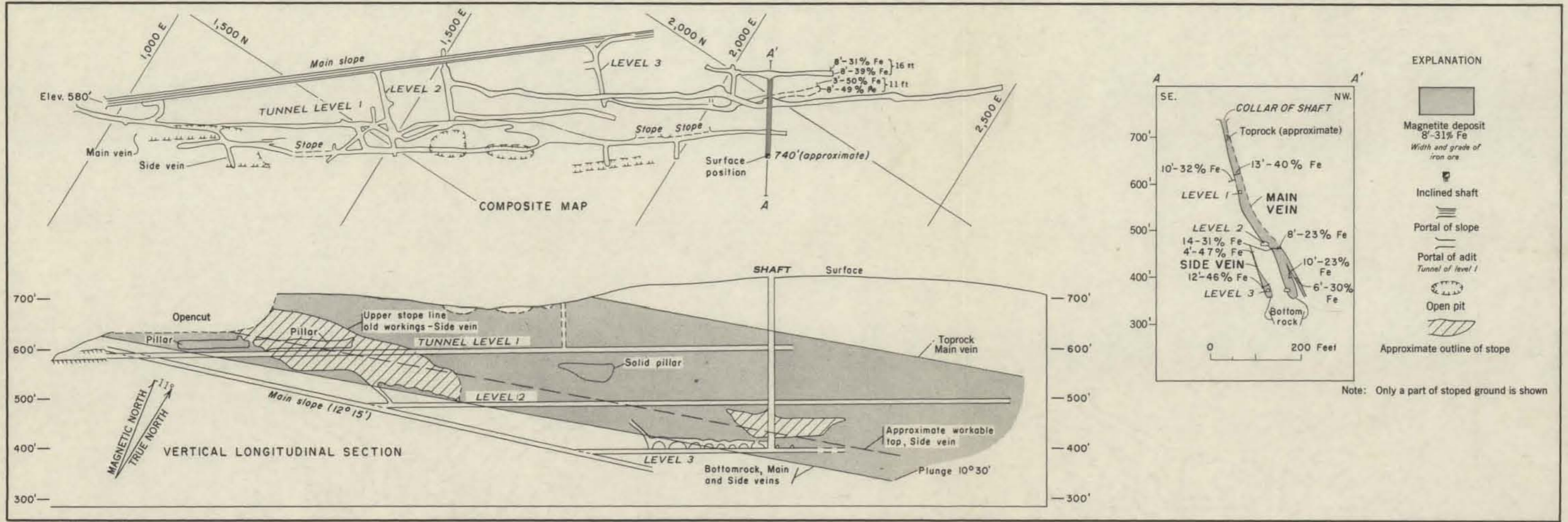
MAP AND SECTIONS OF BEACH GLEN MINE, MORRIS COUNTY, NEW JERSEY
