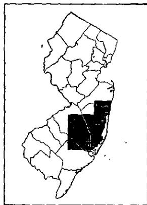
FIG. 10.—Sketch map showing location of the Chatsworth area, New Jersey.
