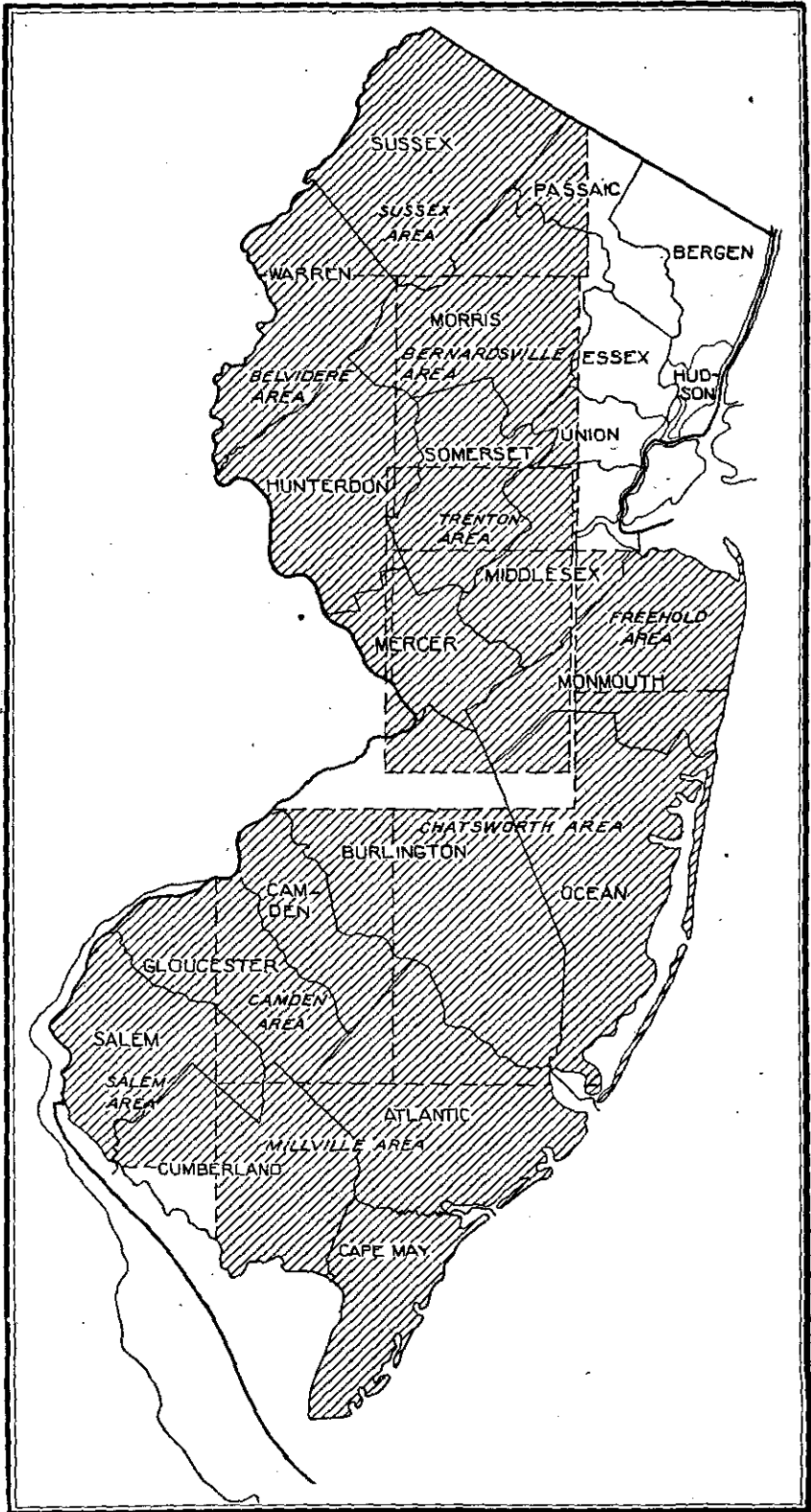
NEW JERSEY GEOLOGICAL SURVEY Areas surveyed in New Jersey, shown by shading.
