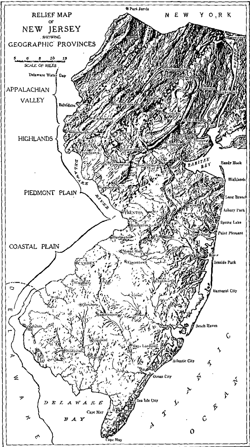
GEOGRAPHIC PROVINCES OF NEW JERSEY.
