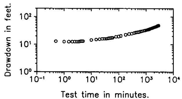
Figure 5. Log-log plot of drawdown in well 14.
