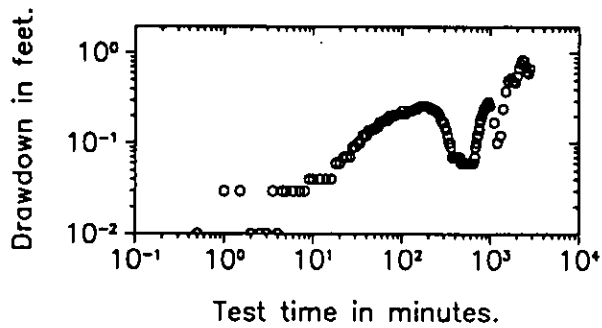
Figure 4. Log-log plot of drawdown in well 13.
