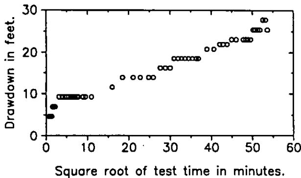
Figure 14. Drawdown plot of well 20 based on the method of Jenkins and Prentice (1982).
