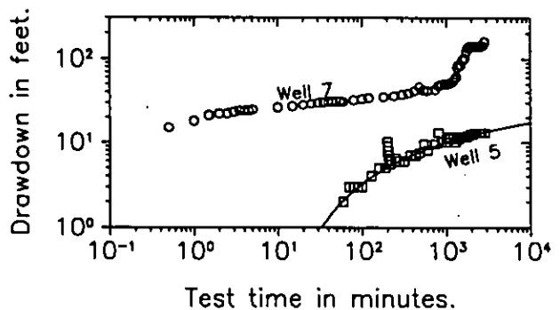
Figure 15. Log-log plot of drawdown in wells 5 and 7.
