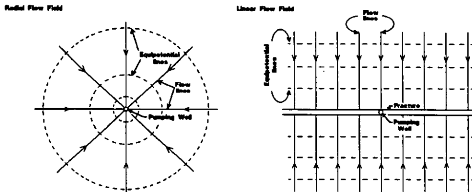
Figure 2. Diagram showing radial and linear flow fields.
