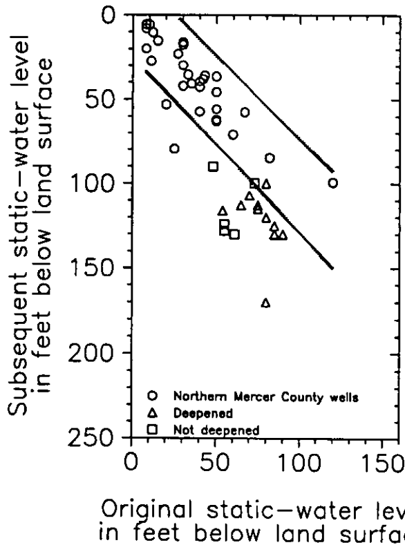
Figure 11. Scatter plot of static-water levels in the Dublin Hills area versus static-water levels in northern Mercer County.
