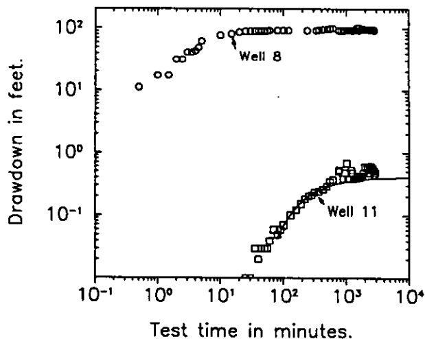
Figure 3. Log-log plot of drawdown in wells 8 and 11.
