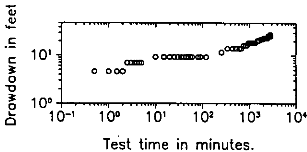
Figure 13. Log-log plot of drawdown in well 20.
