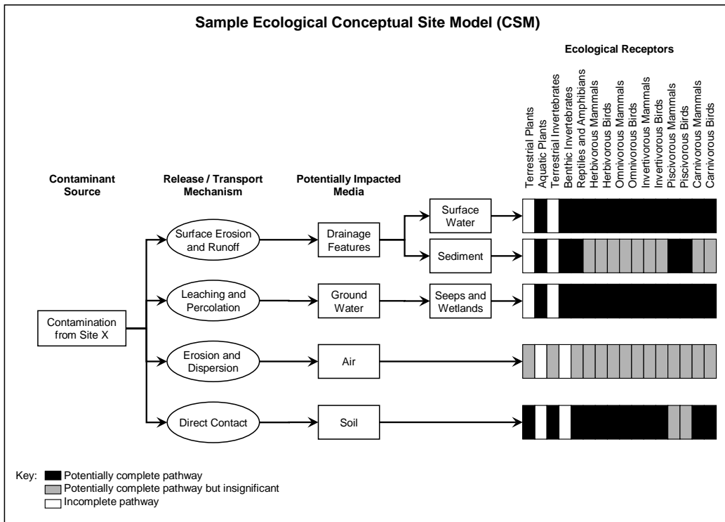
Figure 6-3: Example of an Ecological Conceptual Site Model as a Chart
