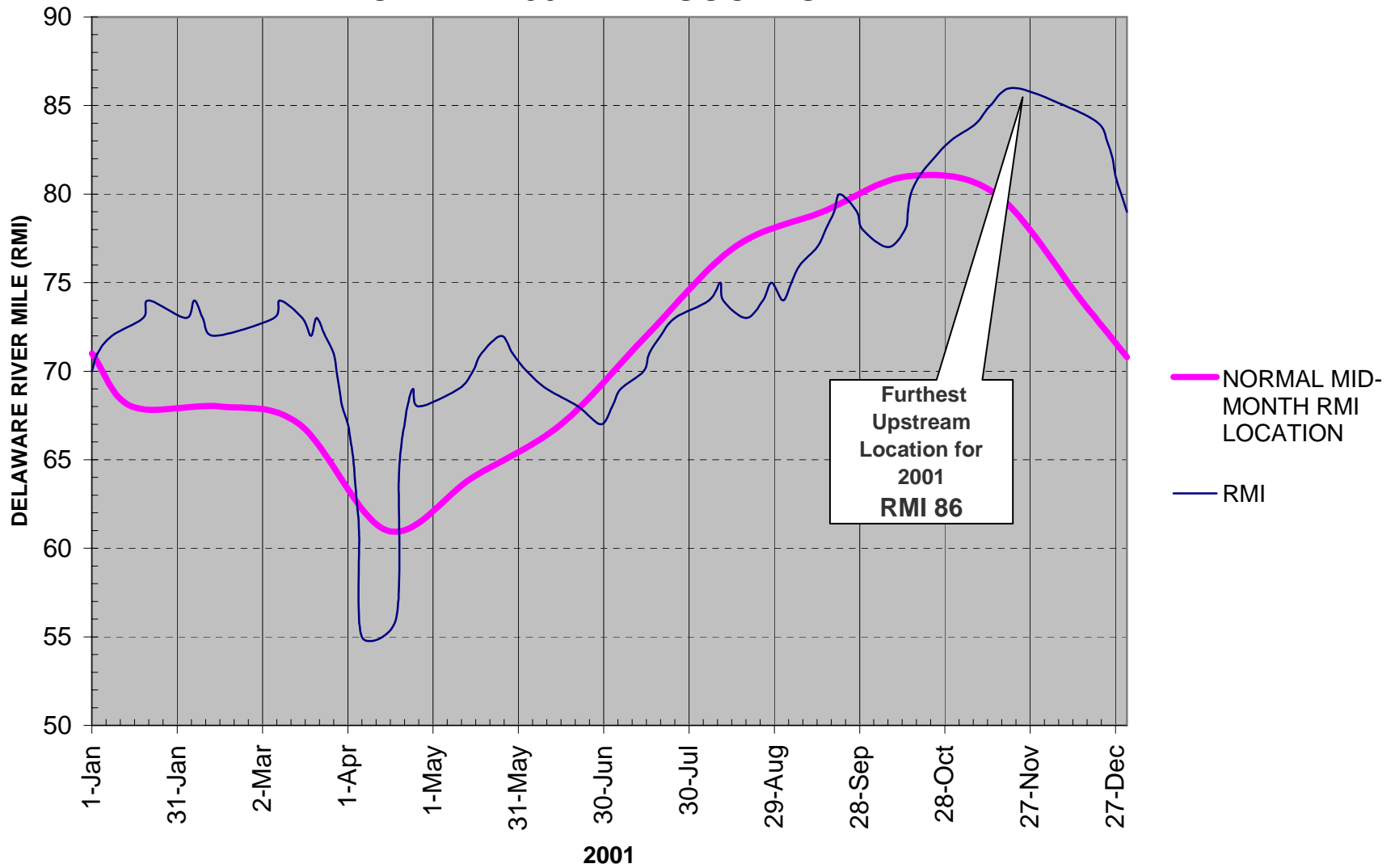
FIGURE 8: LOCATION OF THE 7-DAY AVERAGE OF THE 250-PPM ISOCHLOR
