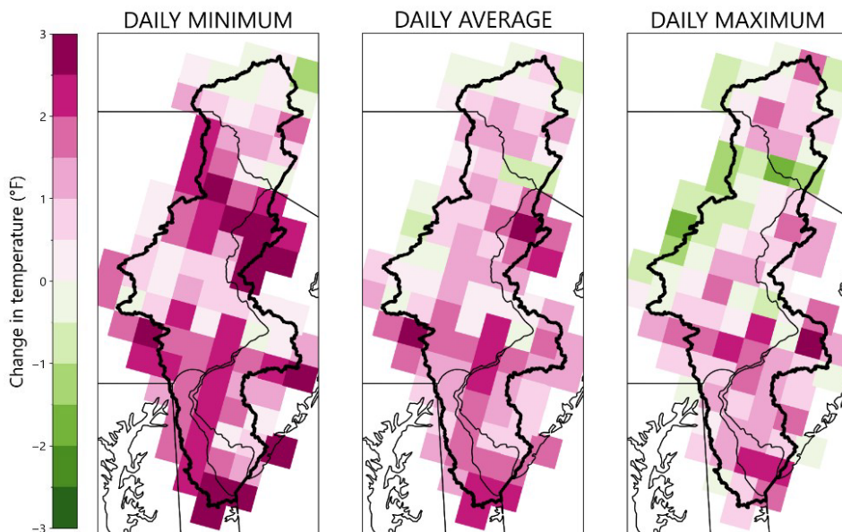
Figure 30. Change in Daily Minimum, Average, and Maximum Temperatures, Comparing the Average over 1950–1979 with 1996–2025. Purple represents increasing temperature and green represents decreasing temperature. Observed data from 370 weather stations were used to generate this gridded temperature dataset for the Basin.
