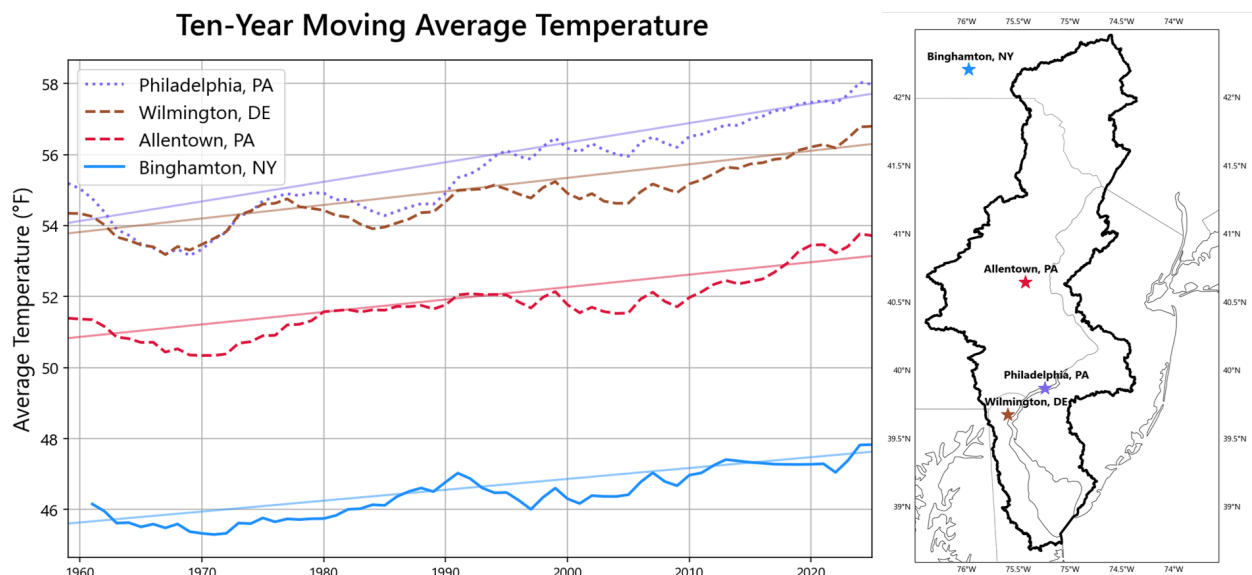
Figure 29. Ten-year moving average of annual temperature at four weather stations in or near the Delaware River Basin. A ten-year moving average is used to show the trend in temperature by “dampening” the interannual variability of weather patterns.
