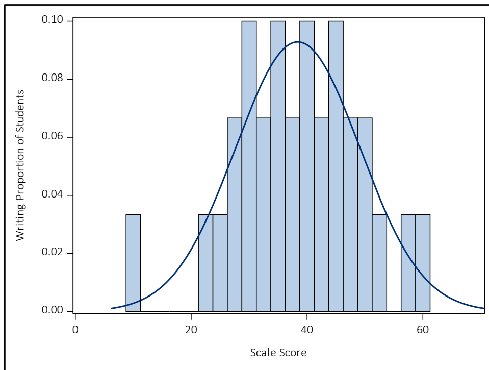
Figure A 7.34 Writing Major Claim Scale Score Distribution for ELA Grade 6
