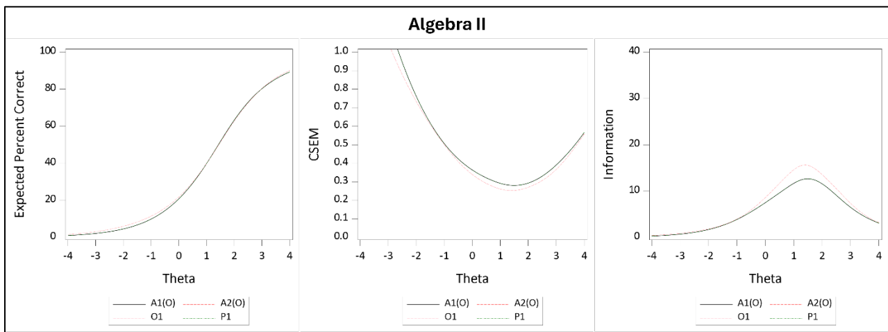
Figure A 7.13 Test Characteristic Curves, CSEM Curves, and Information Curves for Algebra II
