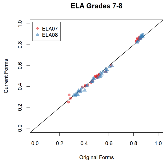
Figure A 10.8 Polyserial Correlations ELA Grades 7–8
