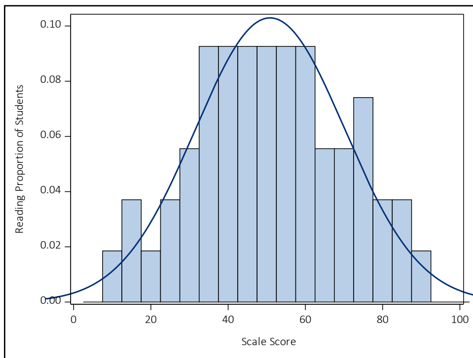
Figure A 7.33 Reading Major Claim Scale Score Distribution for ELA Grade 6
