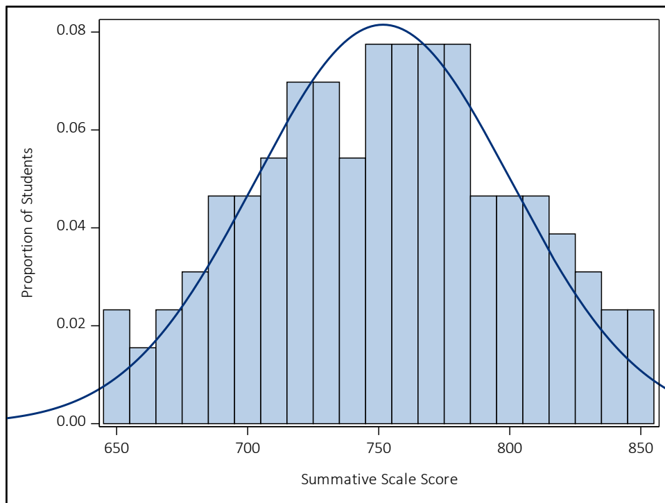
Figure A 7.18 Summative Scale Score Distribution for ELA Grade 7
