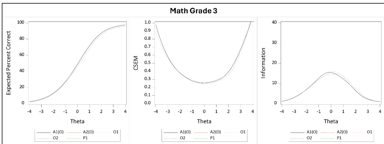
Figure 7.2 Mathematics Grade 3 Test Characteristic Curves, CSEM Curves, and Information Curves
