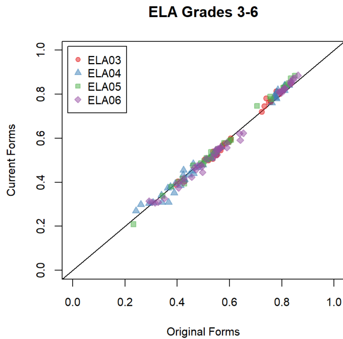
Figure A 10.7 Polyserial Correlations ELA Grades 3–6
