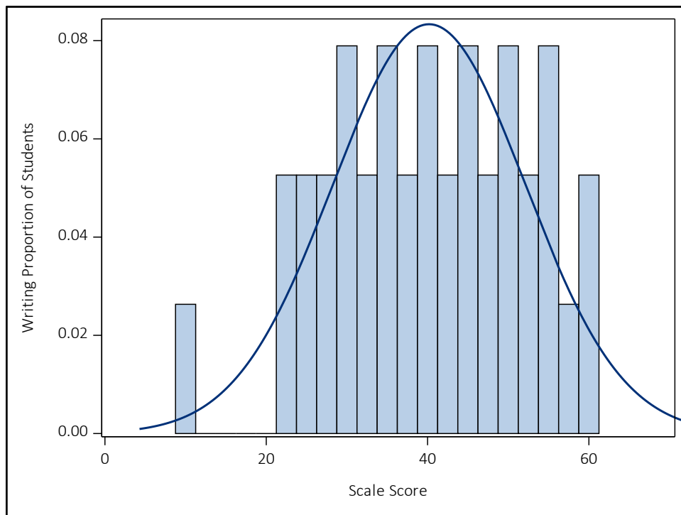
Figure A 7.30 Writing Major Claim Scale Score Distribution for ELA Grade 4
