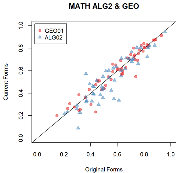
Figure A 10.6 Algebra II and Geometry P-Values
