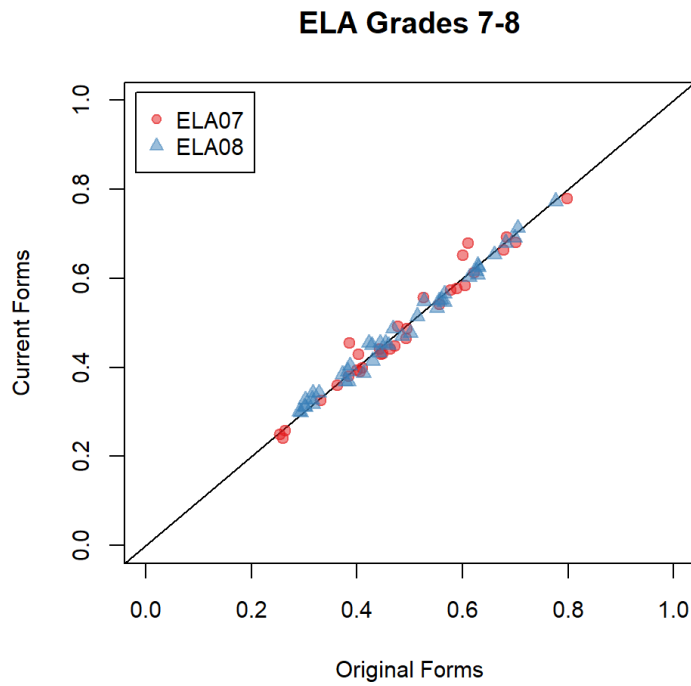
Figure A 10.2 ELA Grades 7–8 P-Values
