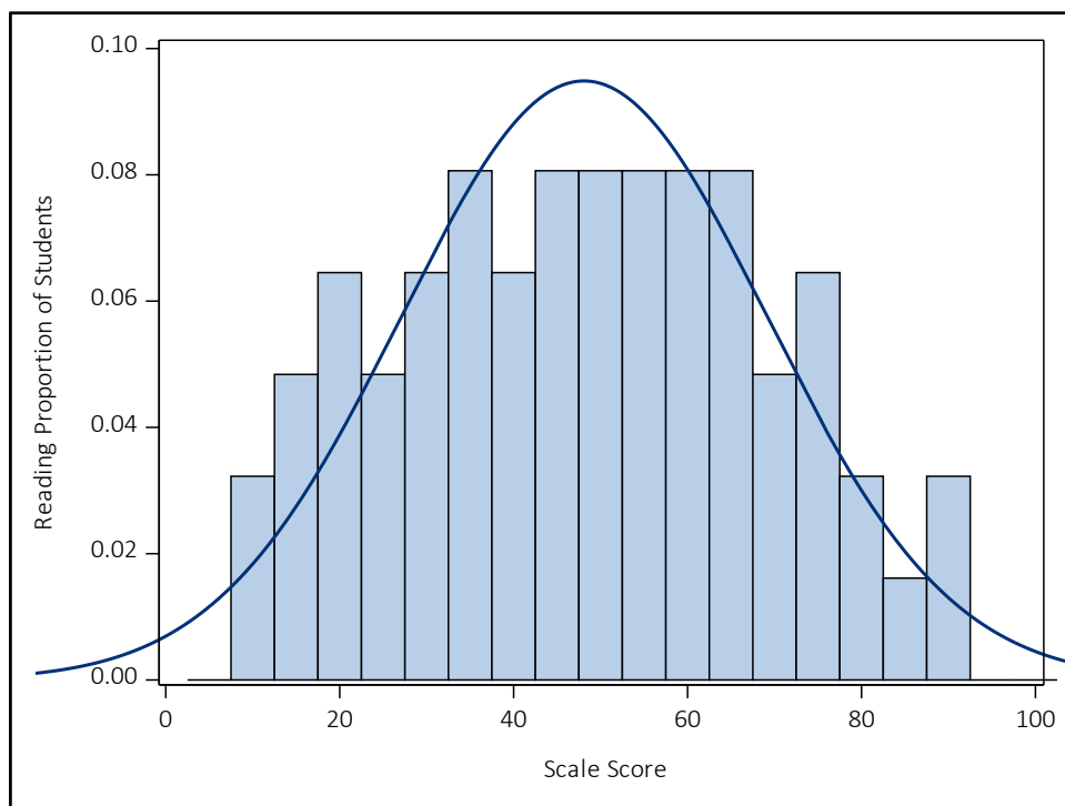
Figure A 7.35 Reading Major Claim Scale Score Distribution for ELA Grade 7
