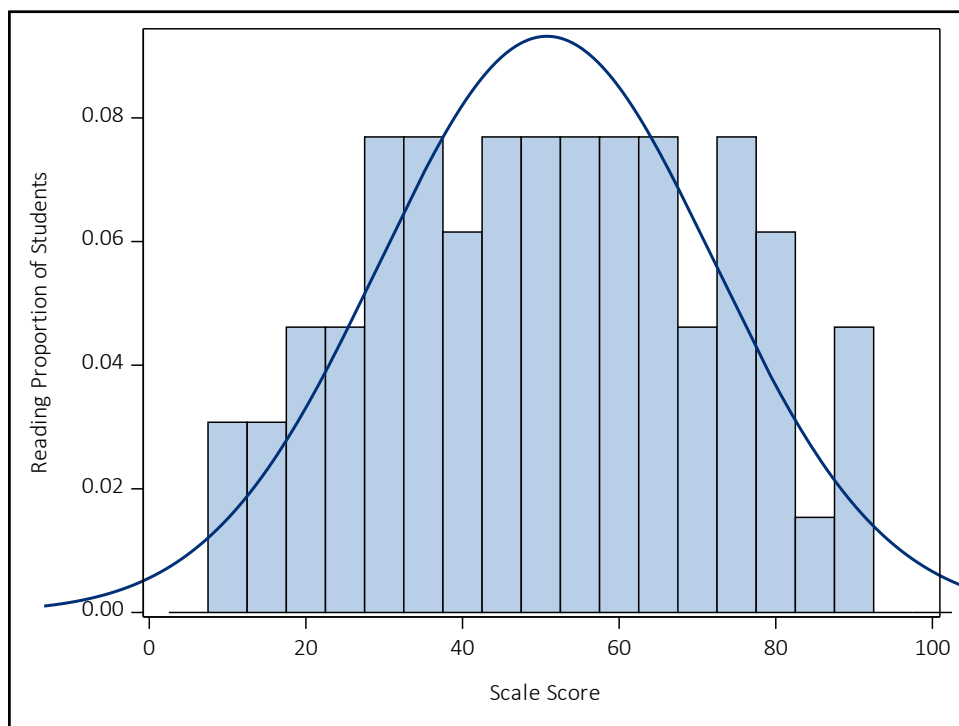
Figure A 7.31 Reading Major Claim Scale Score Distribution for ELA Grade 5
