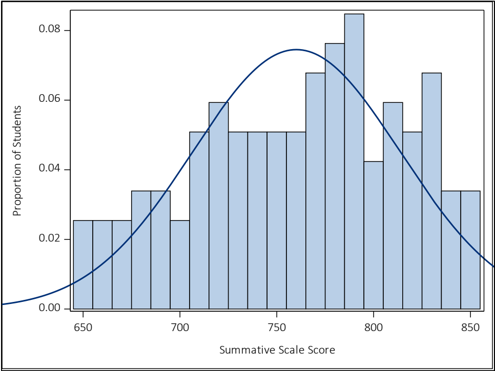
Figure A 7.15 Summative Scale Score Distribution for ELA Grade 4
