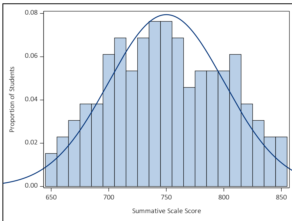
Figure A 7.19 Summative Scale Score Distribution for ELA Grade 8
