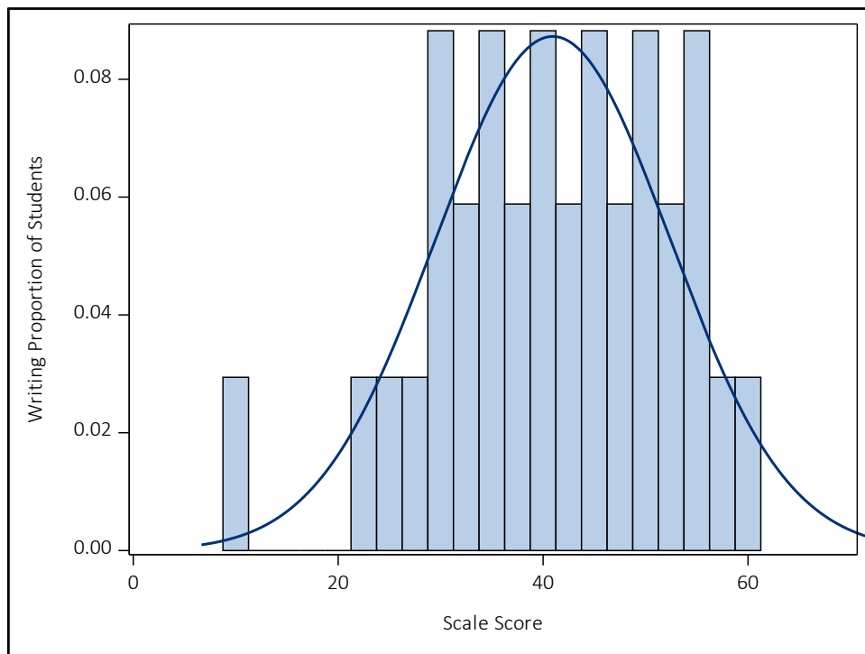
Figure A 7.32 Writing Major Claim Scale Score Distribution for ELA Grade 5
