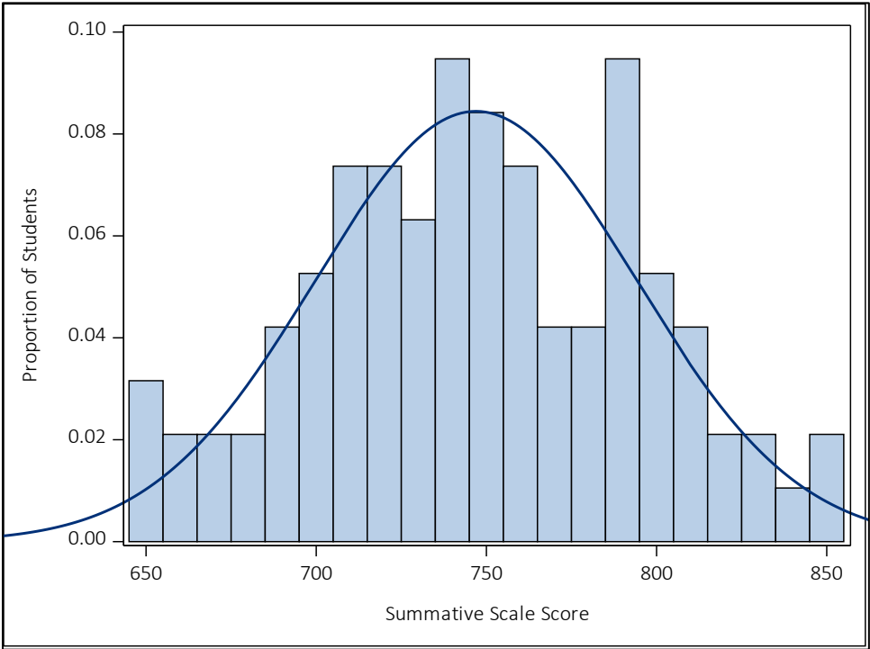
Figure A 7.21 Summative Scale Score Distribution for Mathematics Grade 4
