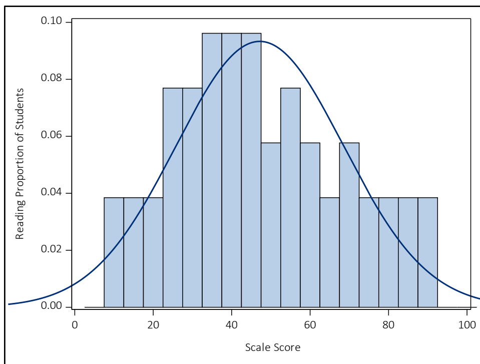
Figure 7.5 Grade 3 ELA Reading Score Distribution
