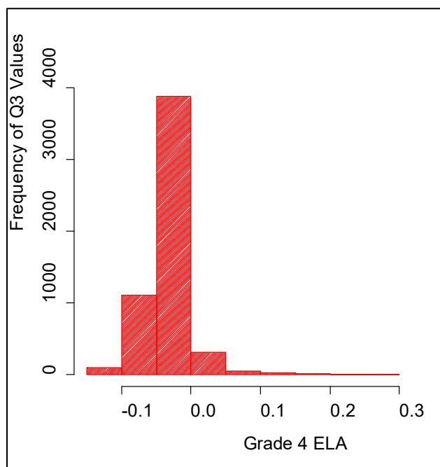
Figure 10.2 Distribution of Q3 Values for Grade 4 ELA (Spring 2015)
