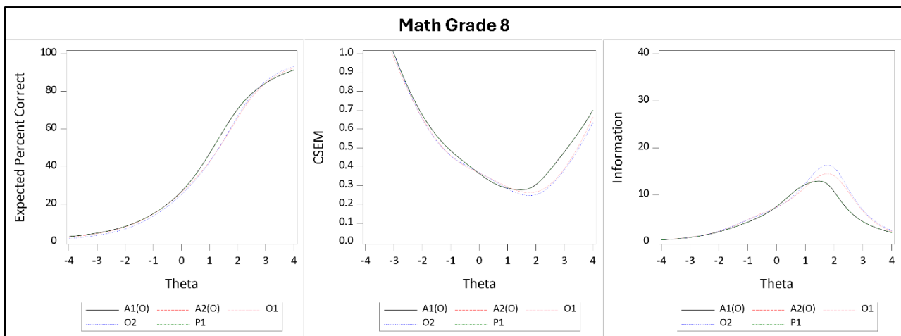
Figure A 7.11 Test Characteristic Curves, CSEM Curves, and Information Curves for Math Grade 8
