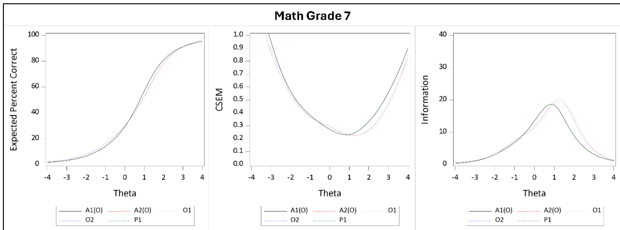
Figure A 7.10 Test Characteristic Curves, CSEM Curves, and Information Curves for Math Grade 7
