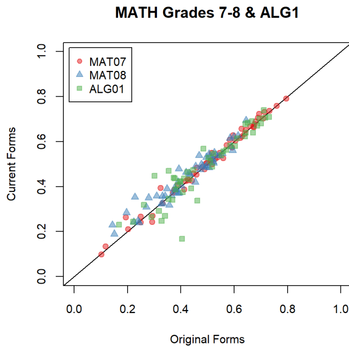
Figure A 10.11 Polyserial Correlations Mathematics Grades 7–8 and Algebra I
