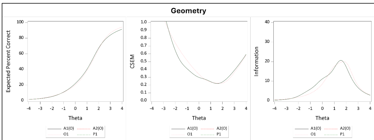
Figure A 7.14 Test Characteristic Curves, CSEM Curves, and Information Curves for Geometry
