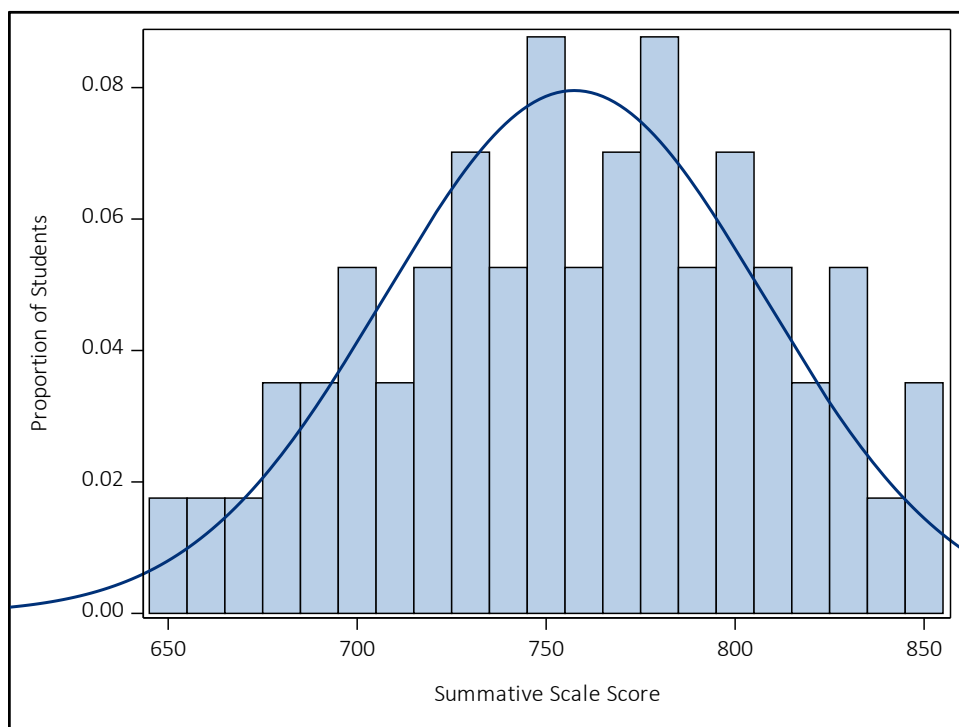
Figure A 7.27 Summative Scale Score Distribution for Algebra II
