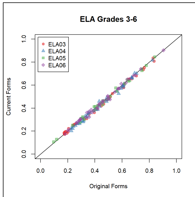
Figure 10.4 ELA Grades 3–6 P-Values
