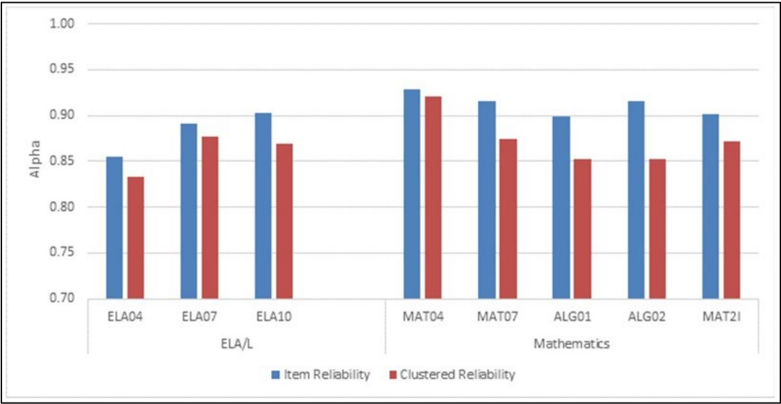
Figure 10.1 Comparison of Internal Consistency by Item and Cluster (Testlet)
