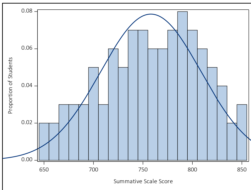
Figure A 7.25 Summative Scale Score Distribution for Mathematics Grade 8
