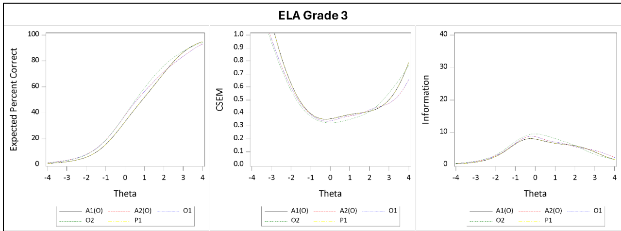
Figure 7.1 ELA Grade 3 Test Characteristic Curves, CSEM Curves, and Information Curves
