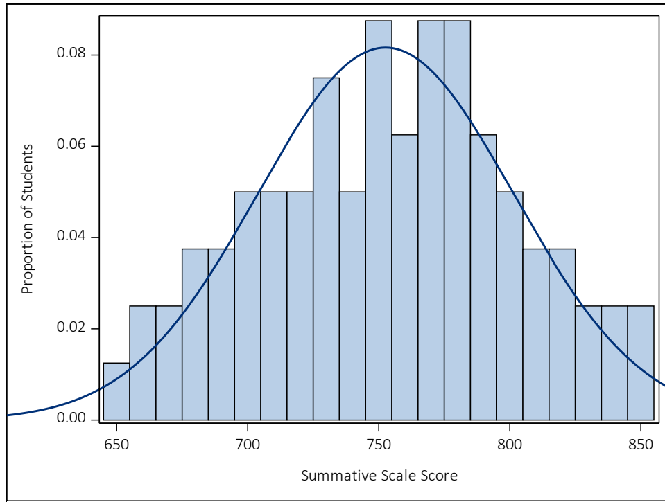
Figure A 7.20 Summative Scale Score Distribution for ELA Grade 9
