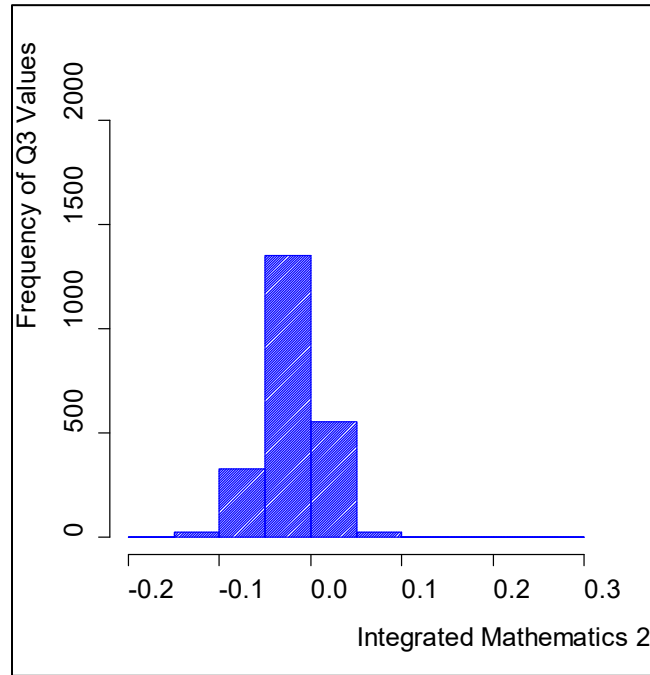
Figure 10.3 Distribution of Q3 Values for Integrated Mathematics II (Spring 2015)
