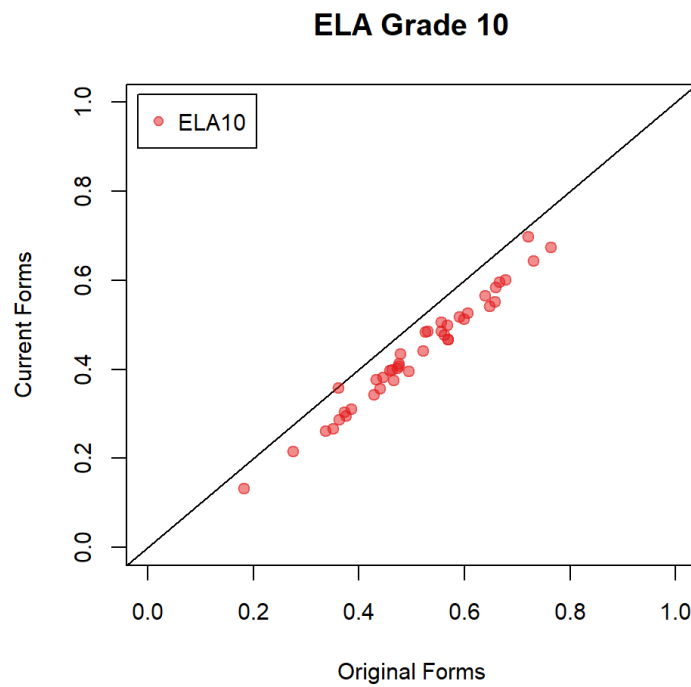
Figure A 10.3 ELA Grade 10 P-Values
