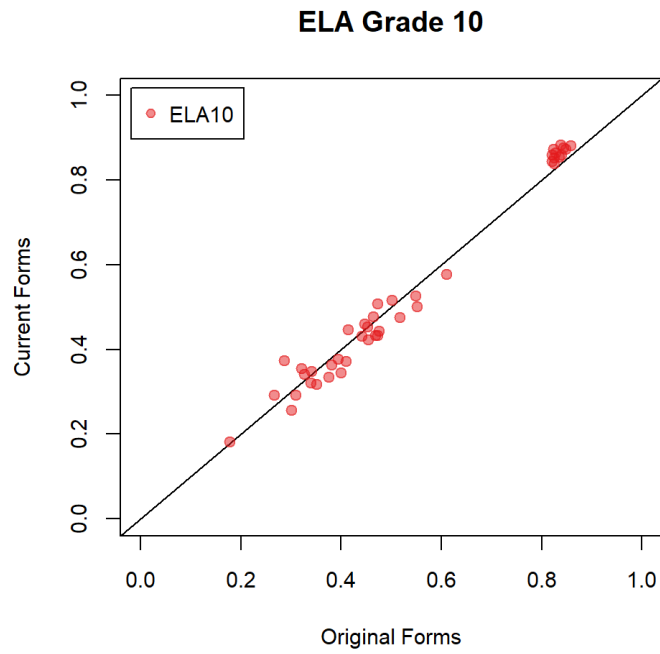
Figure A 10.9 Polyserial Correlations ELA Grade 10
