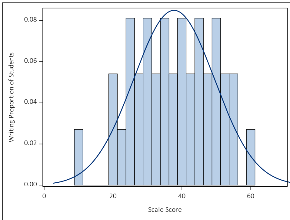
Figure A 7.38 Writing Major Claim Scale Score Distribution for ELA Grade 8
