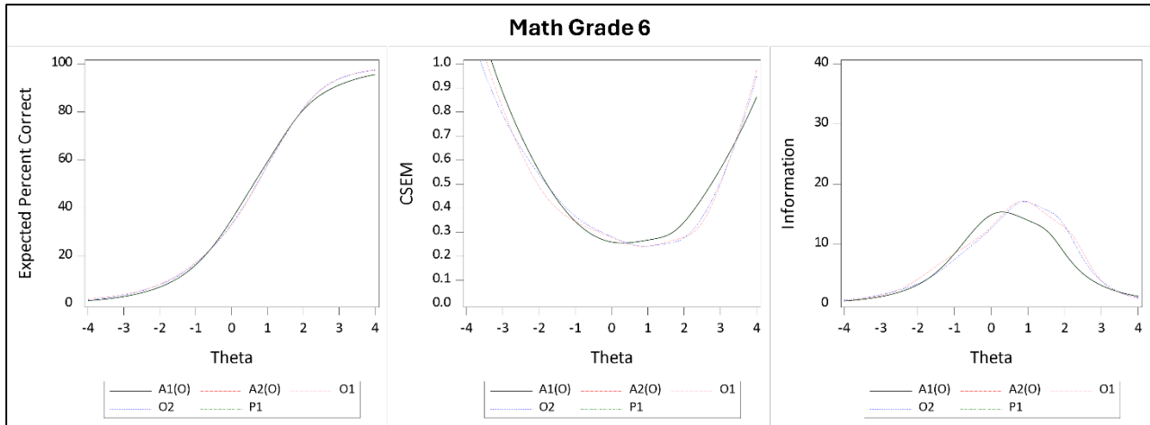
Figure A 7.9 Test Characteristic Curves, CSEM Curves, and Information Curves for Math Grade 6
