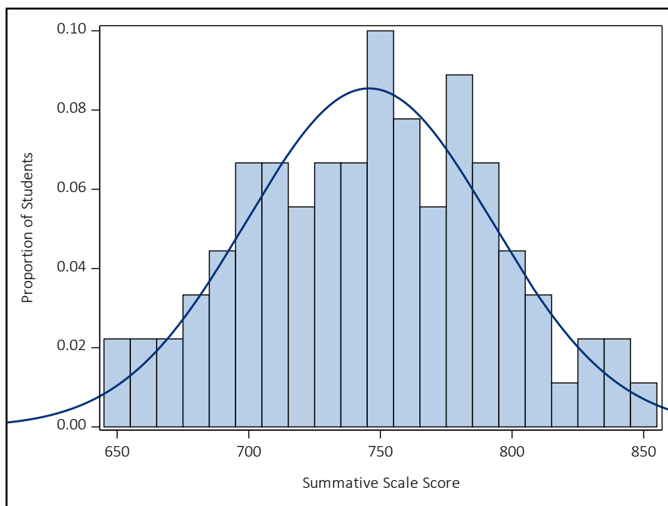
Figure A 7.23 Summative Scale Score Distribution for Mathematics Grade 6
