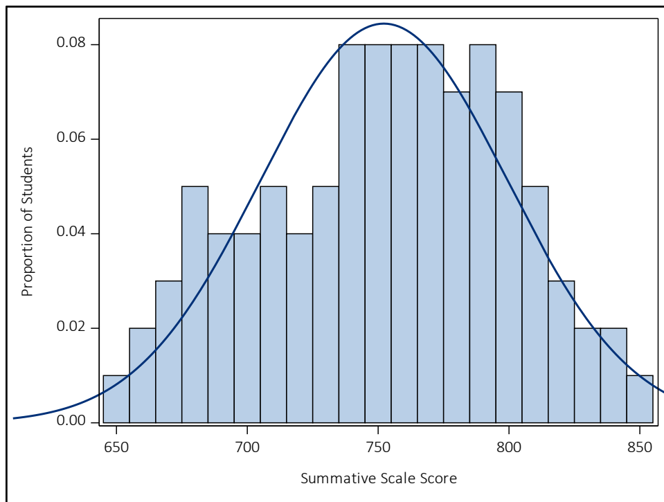
Figure A 7.22 Summative Scale Score Distribution for Mathematics Grade 5
