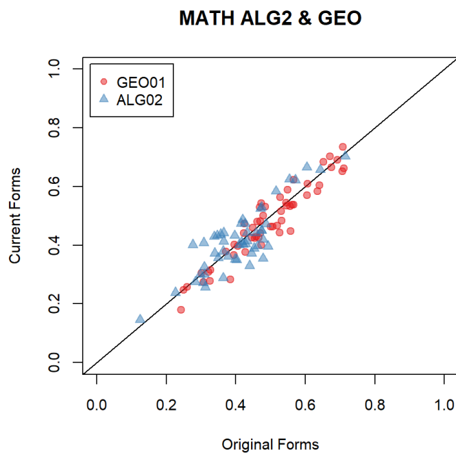
Figure A 10.12 Polyserial Correlations Algebra II and Geometry
