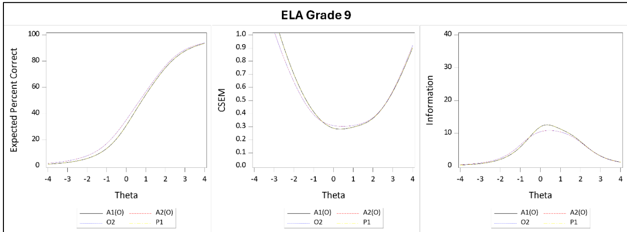
Figure A 7.6 Test Characteristic Curves, CSEM Curves, and Information Curves for ELA Grade 9
