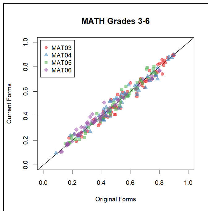
Figure 10.5 Mathematics Grades 3–6 P-Values
