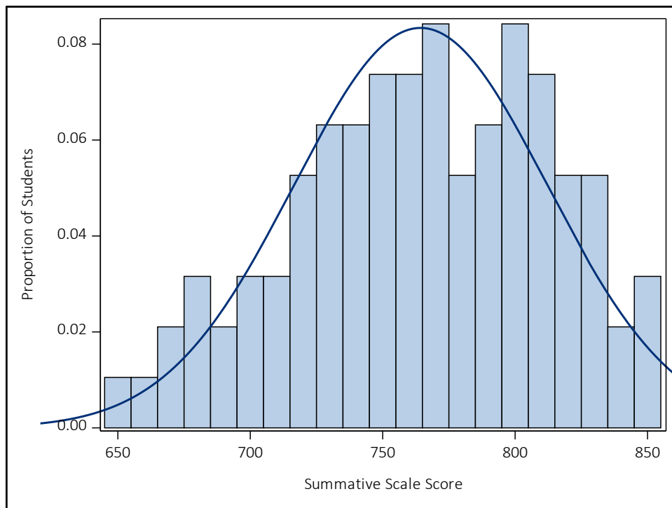
Figure A 7.26 Summative Scale Score Distribution for Algebra I
