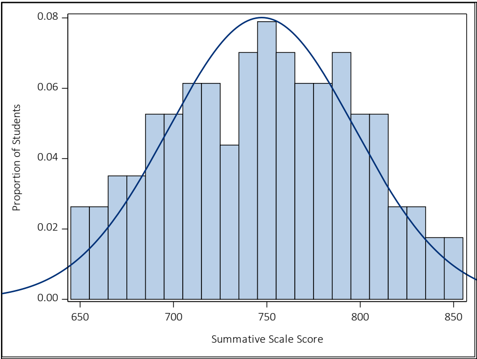
Figure 7.4 Grade 3 Mathematics Score Distribution
