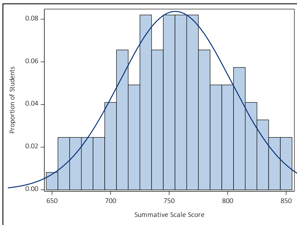
Figure A 7.17 Summative Scale Score Distribution for ELA Grade 6
