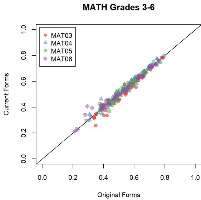
Figure A 10.10 Polyserial Correlations Mathematics Grades 3–6
