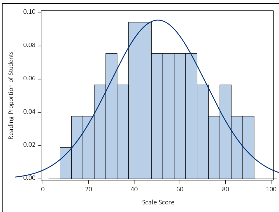
Figure A 7.39 Reading Major Claim Scale Score Distribution for ELA Grade 9
