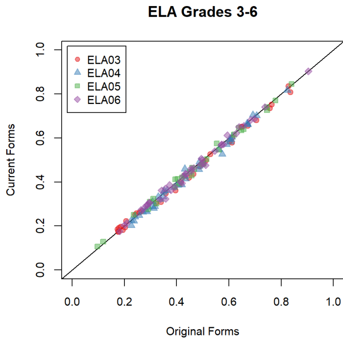
Figure A 10.1 ELA Grades 3–6 P-Values
