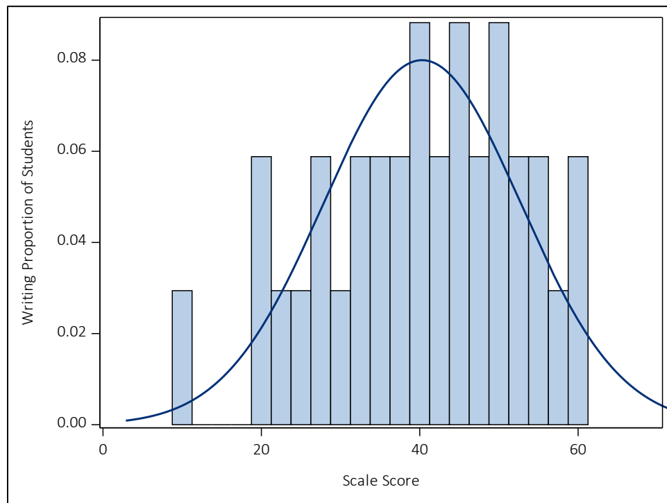
Figure 7.6 Grade 3 ELA Writing Score Distribution
