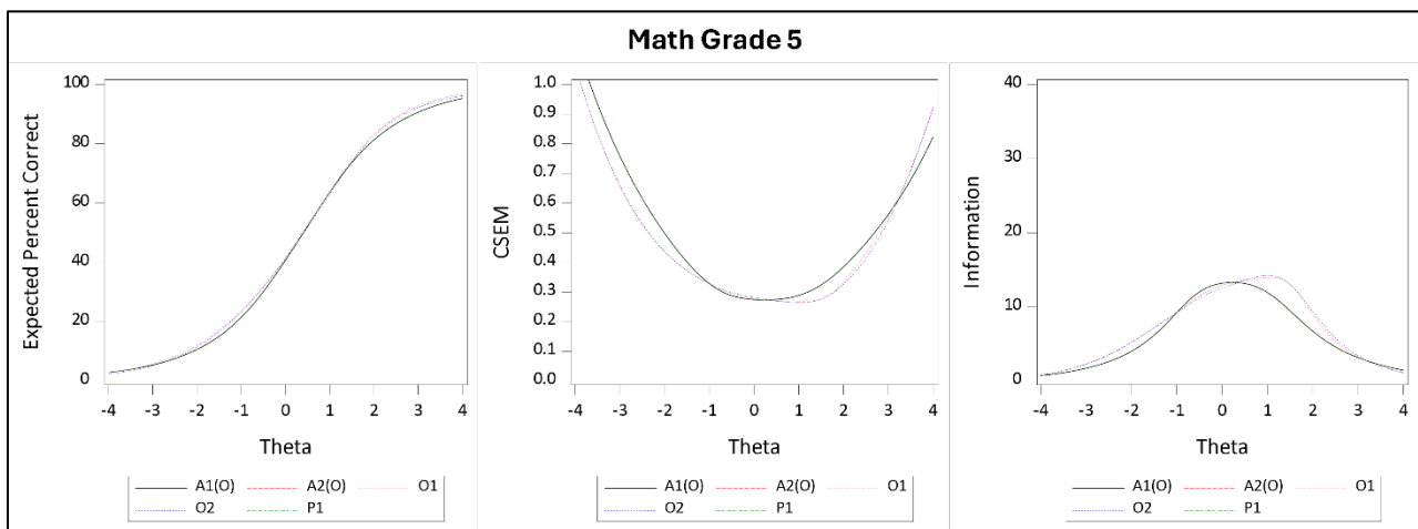
Figure A 7.8 Test Characteristic Curves, CSEM Curves, and Information Curves for Math Grade 5
