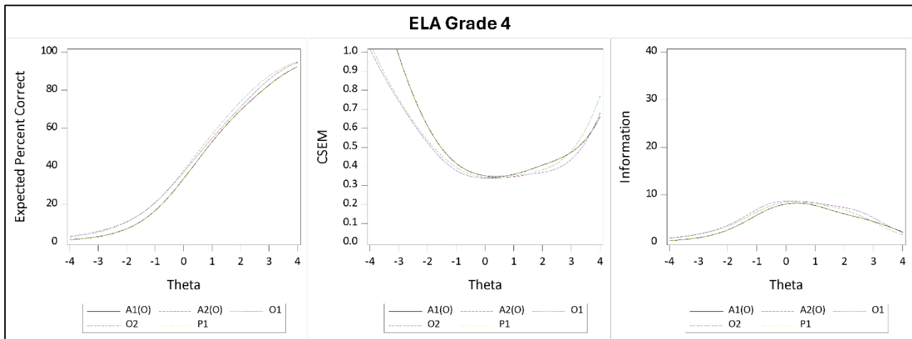
Figure A 7.1 Test Characteristic Curves, CSEM Curves, and Information Curves for ELA Grade 4
