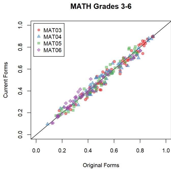
Figure A 10.4 Mathematics Grades 3–6 P-Values
