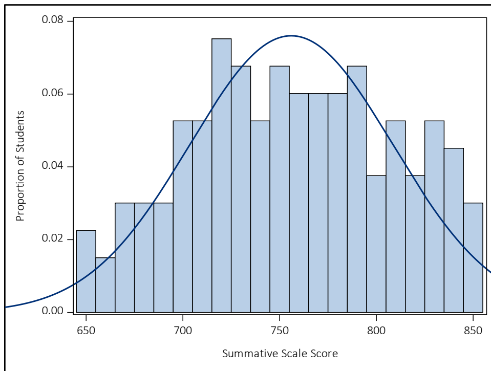
Figure A 7.16 Summative Scale Score Distribution for ELA Grade 5
