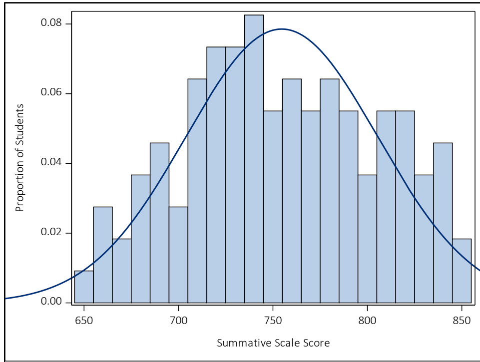
Figure 7.3 Grade 3 ELA Score Distribution
