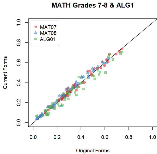
Figure A 10.5 Mathematics Grade 7–8 and Algebra I P-Values
