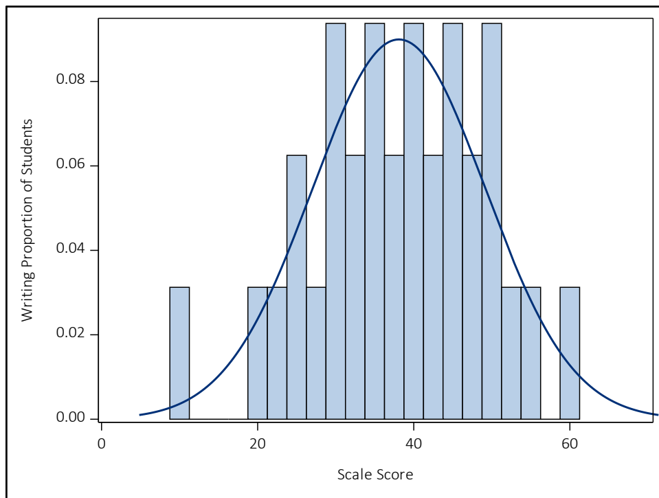
Figure A 7.40 Writing Major Claim Scale Score Distribution for ELA Grade 9
