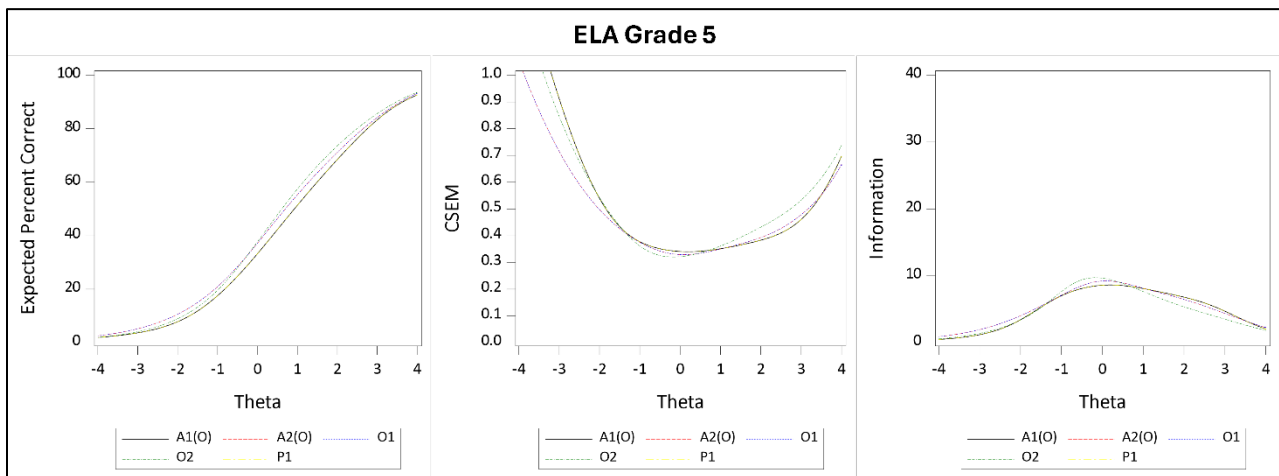
Figure A 7.2 Test Characteristic Curves, CSEM Curves, and Information Curves for ELA Grade 5
