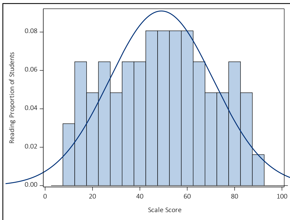
Figure A 7.37 Reading Major Claim Scale Score Distribution for ELA Grade 8
