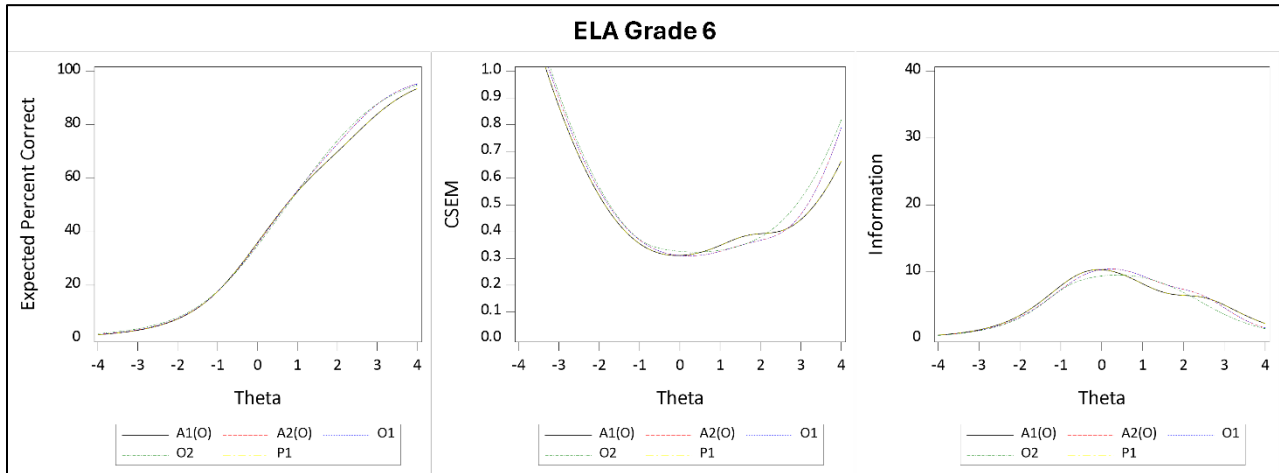
Figure A 7.3 Test Characteristic Curves, CSEM Curves, and Information Curves for ELA Grade 6
