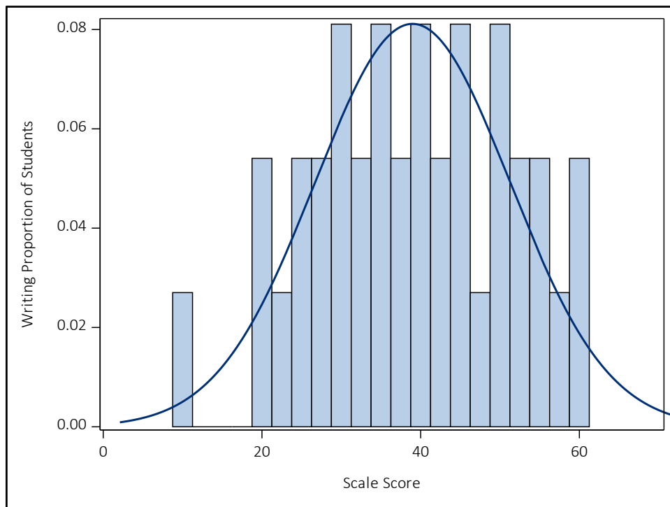
Figure A 7.36 Writing Major Claim Scale Score Distribution for ELA Grade 7
