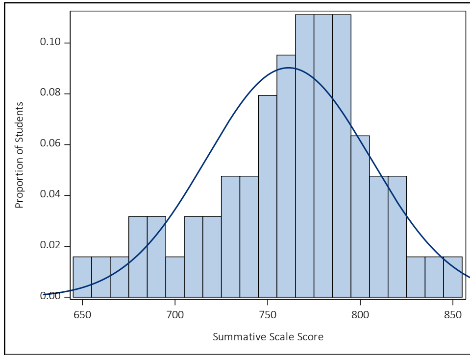
Figure A 7.28 Summative Scale Score Distribution for Geometry
