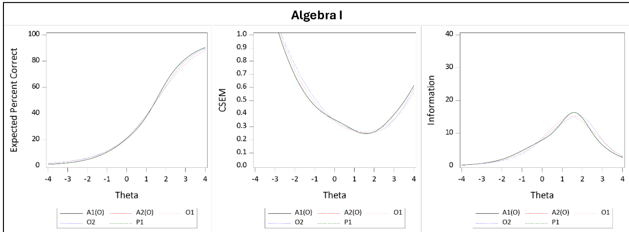
Figure A 7.12 Test Characteristic Curves, CSEM Curves, and Information Curves for Algebra I
