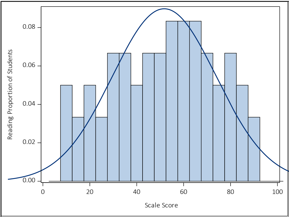
Figure A 7.29 Reading Major Claim Scale Score Distribution for ELA Grade 4
