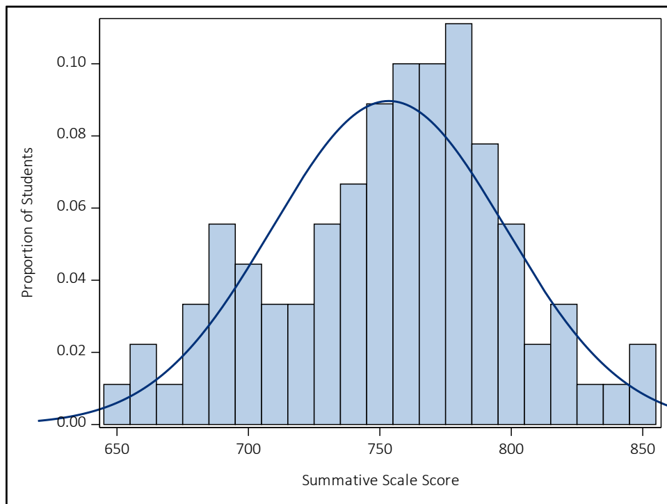
Figure A 7.24 Summative Scale Score Distribution for Mathematics Grade 7
